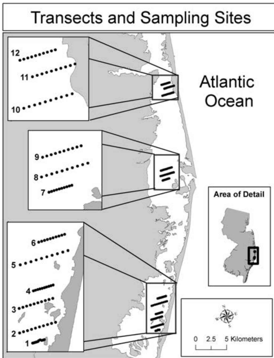
Figure B1-2. Seagrass beds showing 120 sampling stations along 12 estuary transects.
