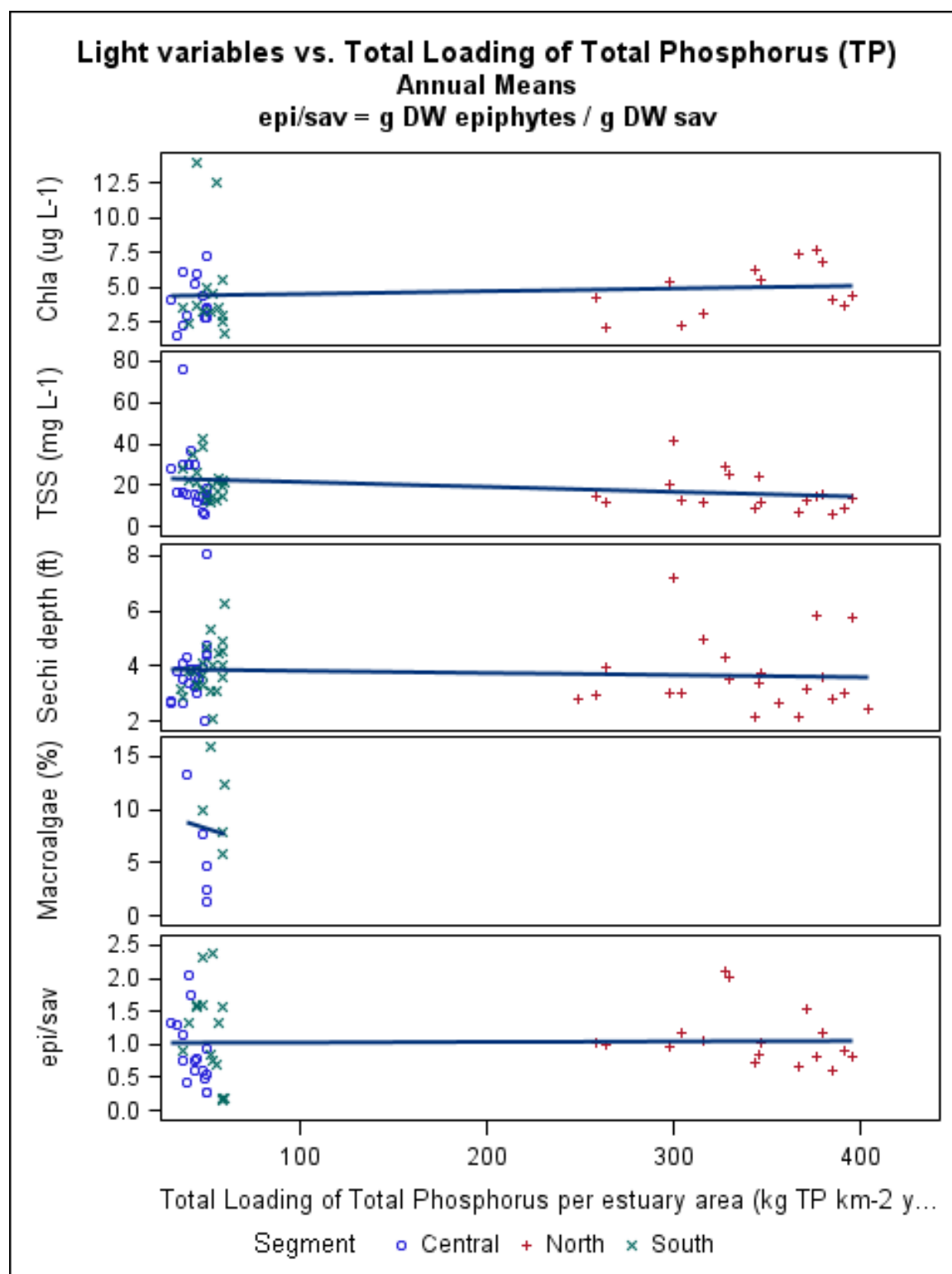
Figure 3 - 19 Light availability indicators vs. total phosphorus loading
