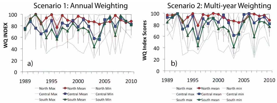
Figure 3 - 45 Weighted Scores under Scenario 1 and Scenario 2 for Water Quality Index.
