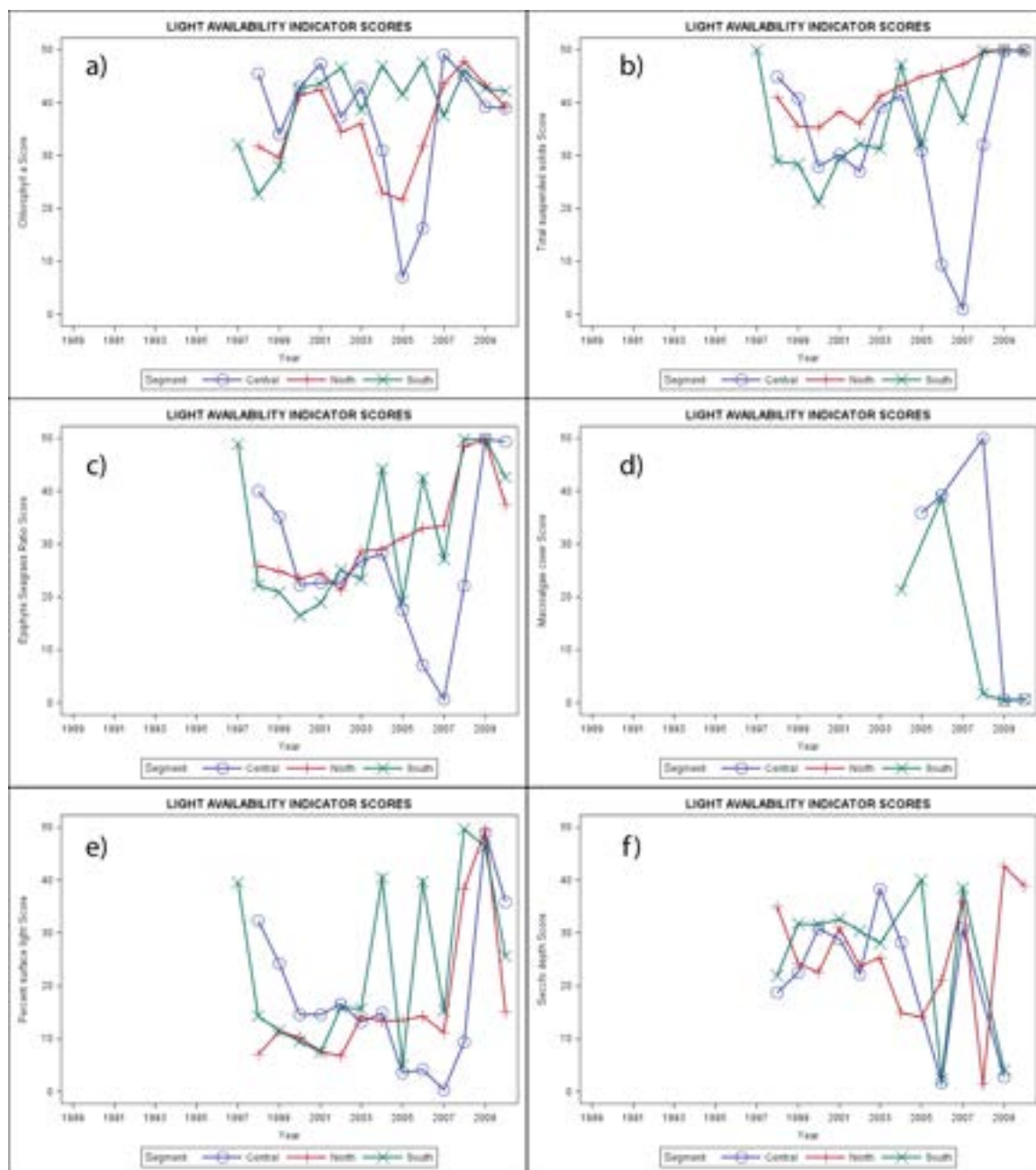
Figure 3 - 50 Scores of Light Availability indicators: (a) chlorophyll, (b) total suspended solids, (c) epiphyte:seagrass ratio, (d) macroalgae cover, (e) percent surface light, (f) Secchi depth.
