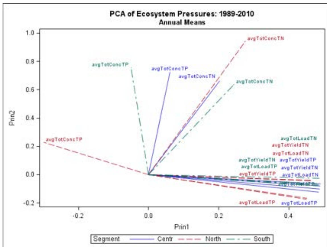
Figure 3 - 3 Principal component analysis of Total Loading, Total Yield, and Flow-weighted average total concentration for total nitrogen and total phosphorus.
