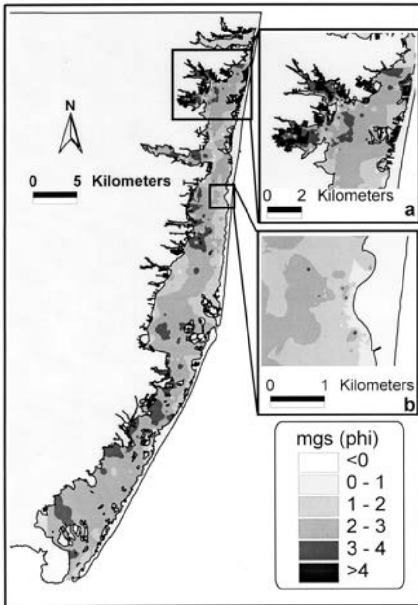
Figure 1 - 7 Bottom sediment composition and distribution (phi units) documented in the estuary. Finer grained sediments (silt, clay, and organic material) derived from upland areas, streams, and wetlands concentrate along the mainland and west side of the estuary. Well-sorted sands of marine origin and the back barrier predominate on the east side of the estuary. Sediment distribution may show a larger area of sediment type than actually exists due to the spacing of sampling locations and occurrence of mosaic patterns. (From Psuty, 2004).
