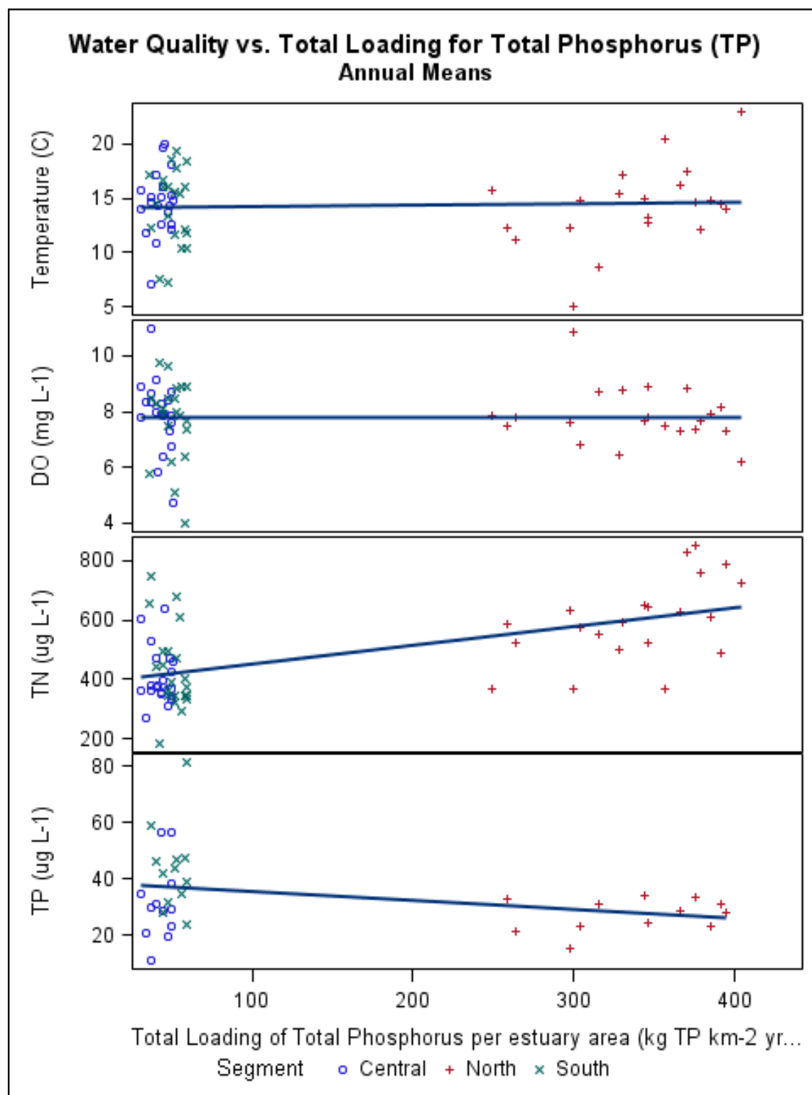
Figure 3 - 18 Water quality indicators vs. total phosphorus loading.
