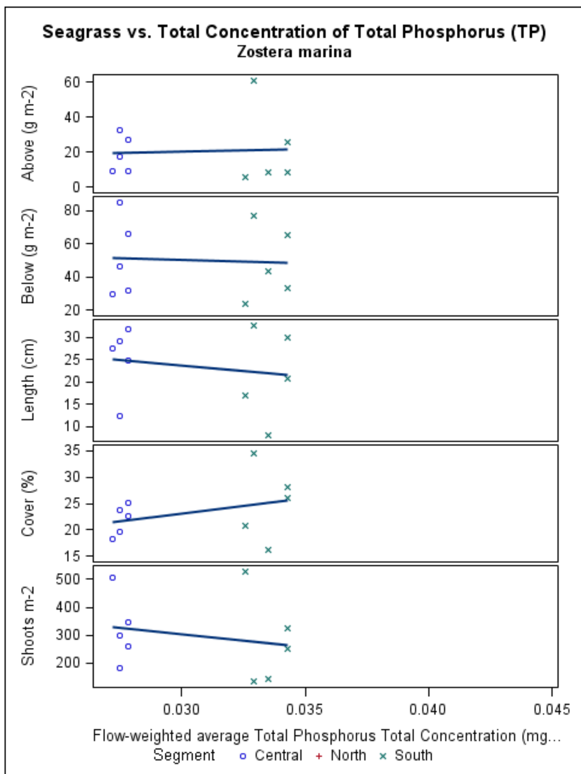
Figure 3 - 7 Zostera marina indicators vs. flow-weighted averaged total concentration of total phosphorus (mg L -1 ).
