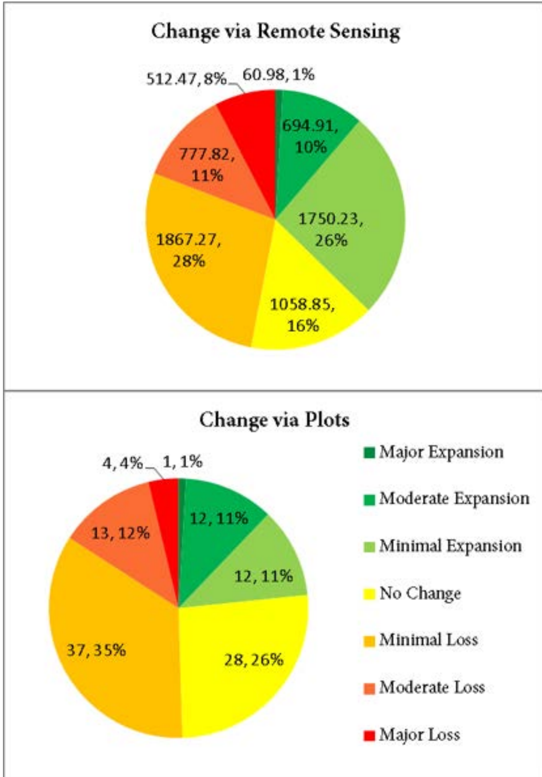
Figure 1. Remotely sensed (2003-2009) vs. in situ plot (2004-2010) change results.
