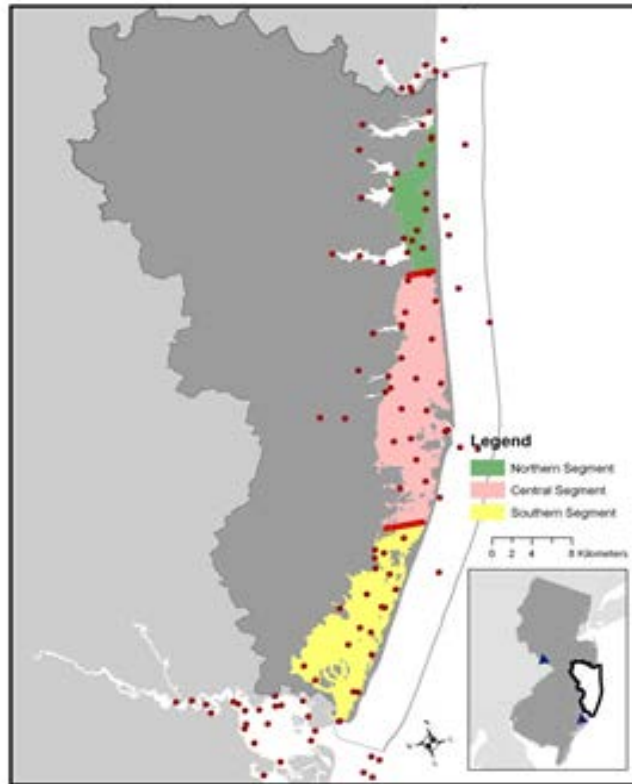
Figure 1 - 5 Map of the BB-LEH Estuary showing three segments (north, central, and south) used for index development.
