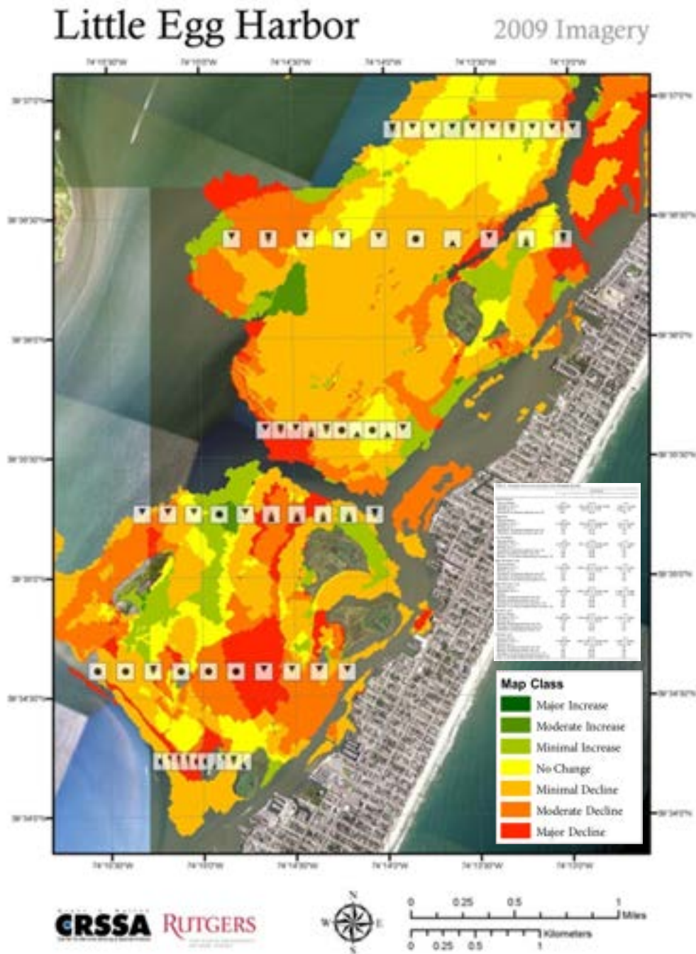
Figure 5. Seagrass 2003-2009 Change map with 2004-2010 plot-based data superimposed for the Little Egg Harbor study sub-area.
