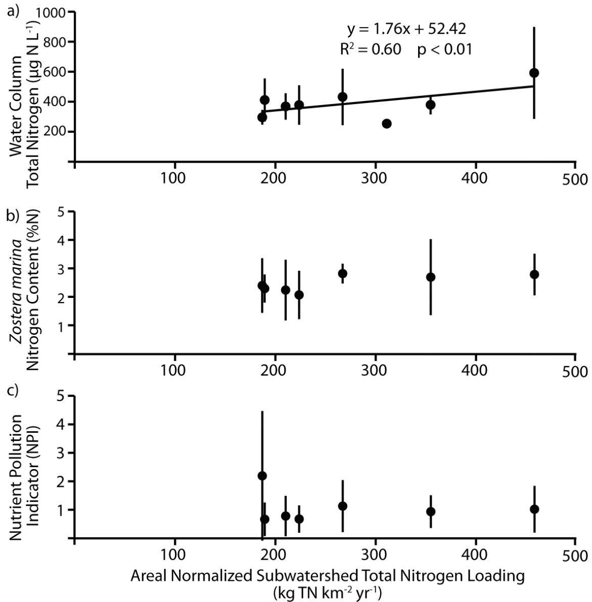
Figure 3 - 13 Estuarine nitrogen concentration, eelgrass nitrogen content, and a 'Nutrient Pollution Indicator' vs nitrogen loading in Barnegat Bay-Little Egg Harbor. (From Kennish and Fertig 2012).
