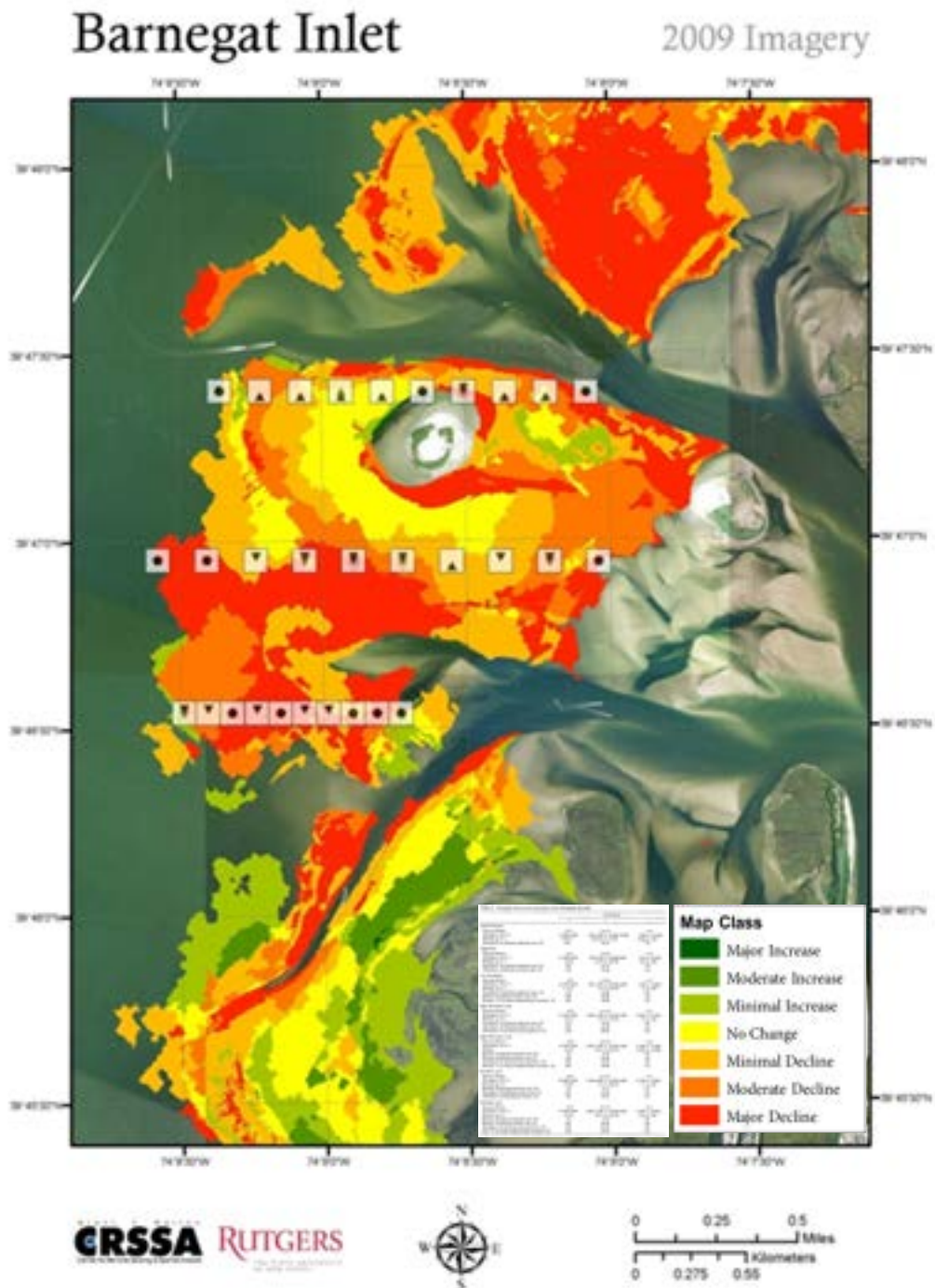
Figure 4. Seagrass 2003-2009 Change map with 2004-2010 plot-based data superimposed for the Barnegat Inlet study sub-area.
