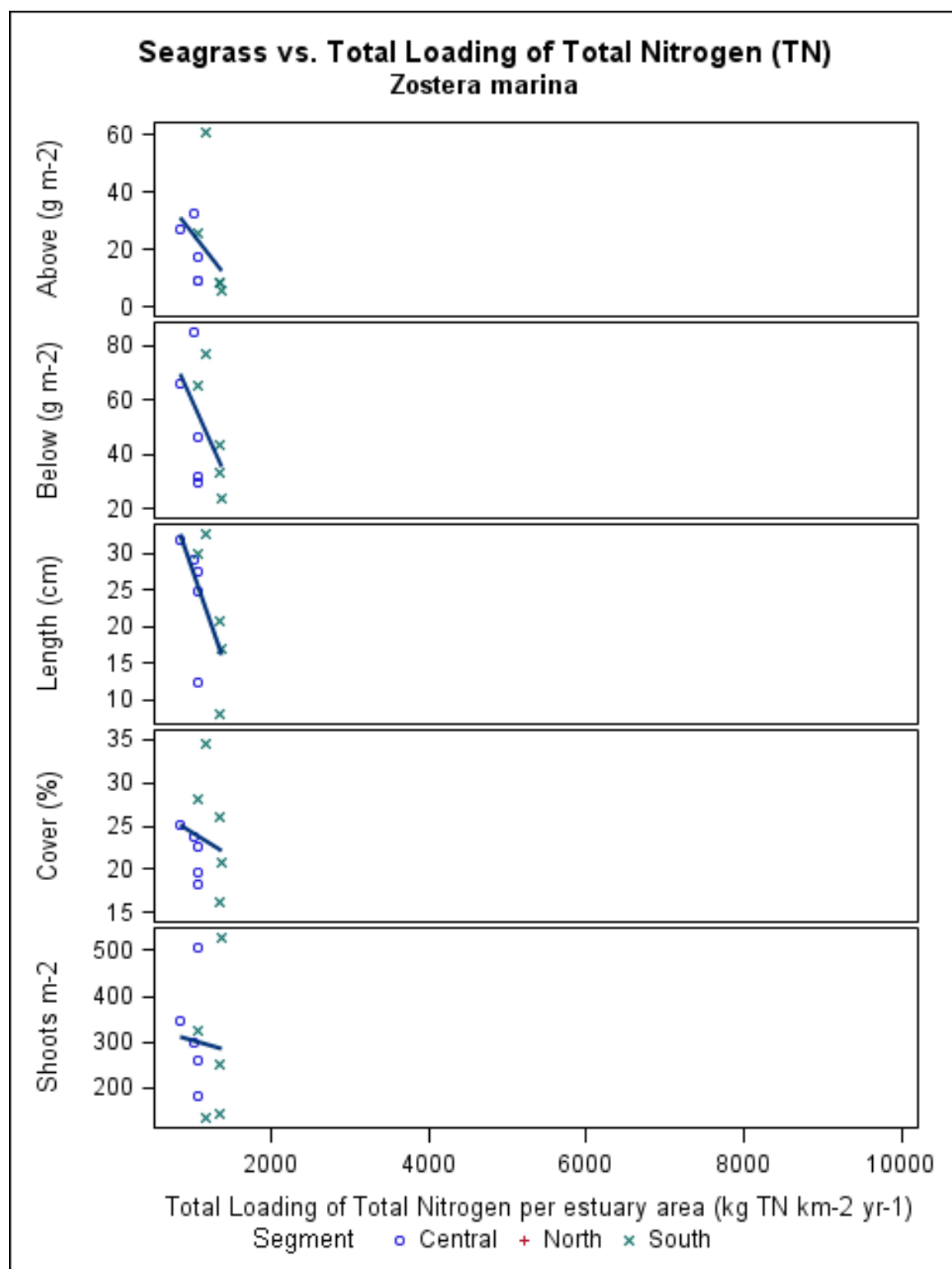
Figure 3 - 17 Seagrass indicators vs total nitrogen loading
