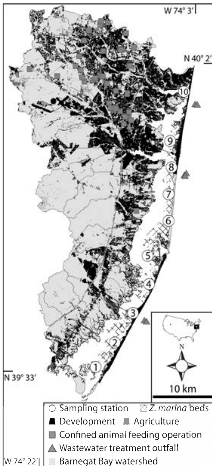
Figure 1 - 4 Land use of BB-LEH watershed. Note locations of 52 confined animal feeding operations.
