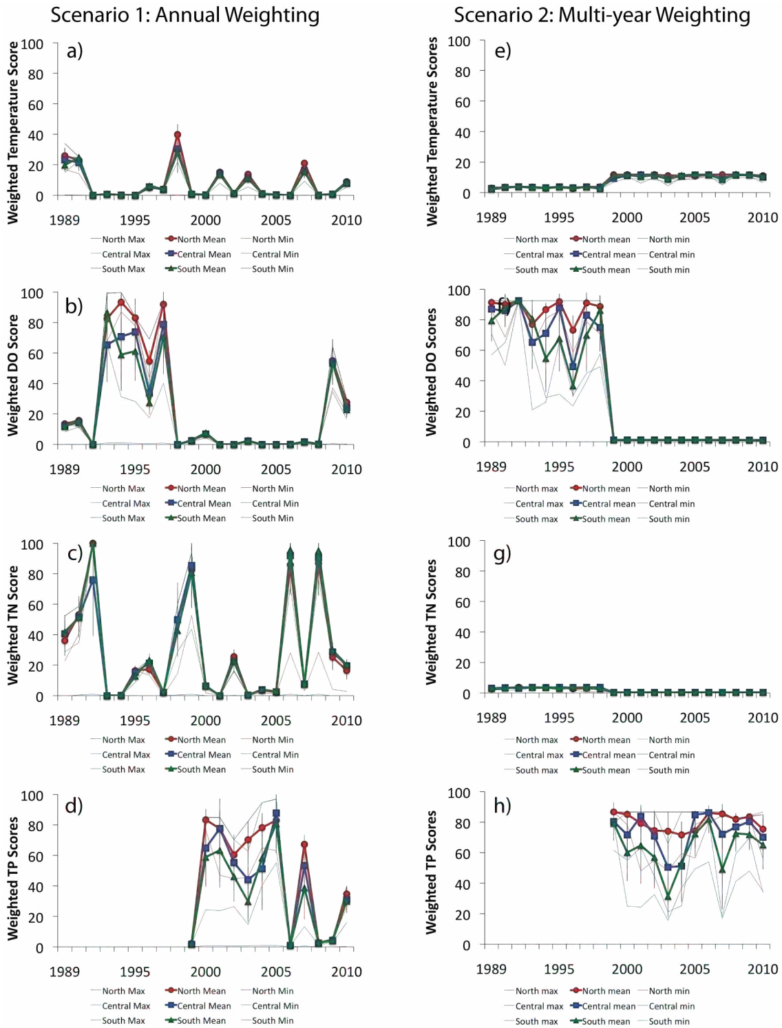
Figure 3 - 44 Weighted scores for water quality under Scenario 1 and Scenario 2.
