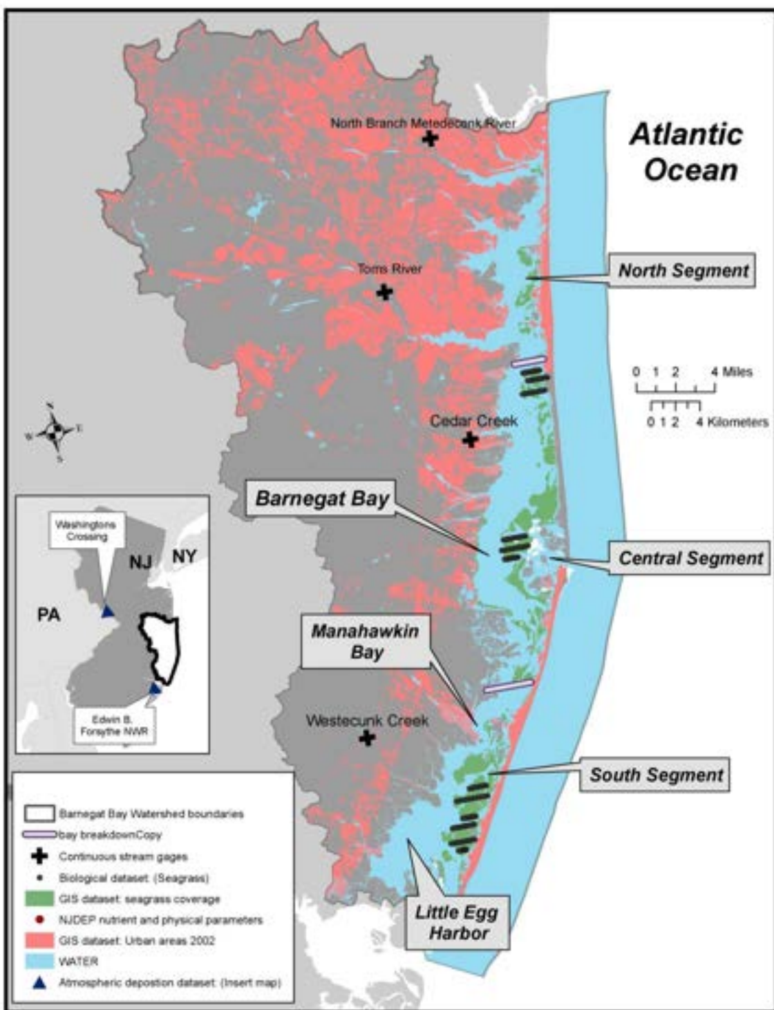
Figure B1-1. Barnegat Bay-Little Egg Harbor Estuary showing north, central, and south sampling segments.
