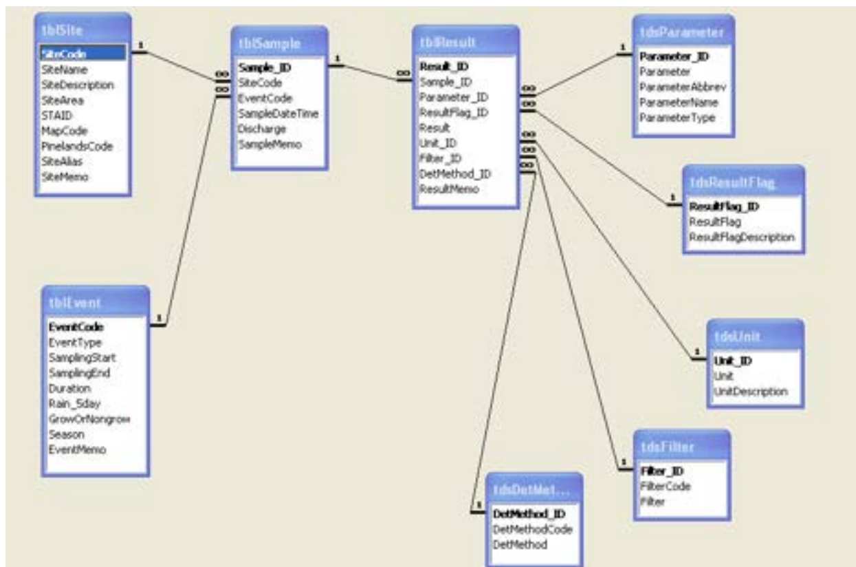
Figure B10-1. Relationships among the data tables in the Access database for secondary data
