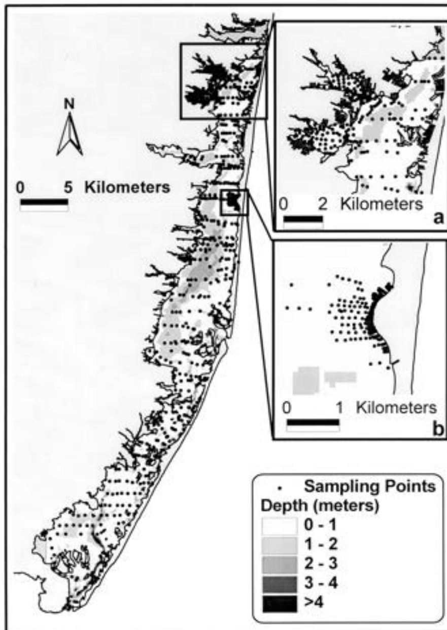
Figure 1 - 6 Map showing a grid of bottom sediment sampling stations and bathymetric measurements in the BB-LEH Estuary. (From Psuty, 2004).
