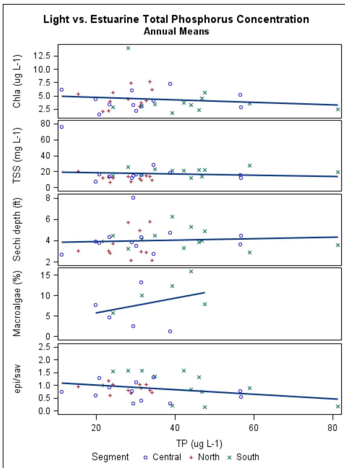
Figure 3 - 30 Light indicators vs estuarine total phosphorus concentration
