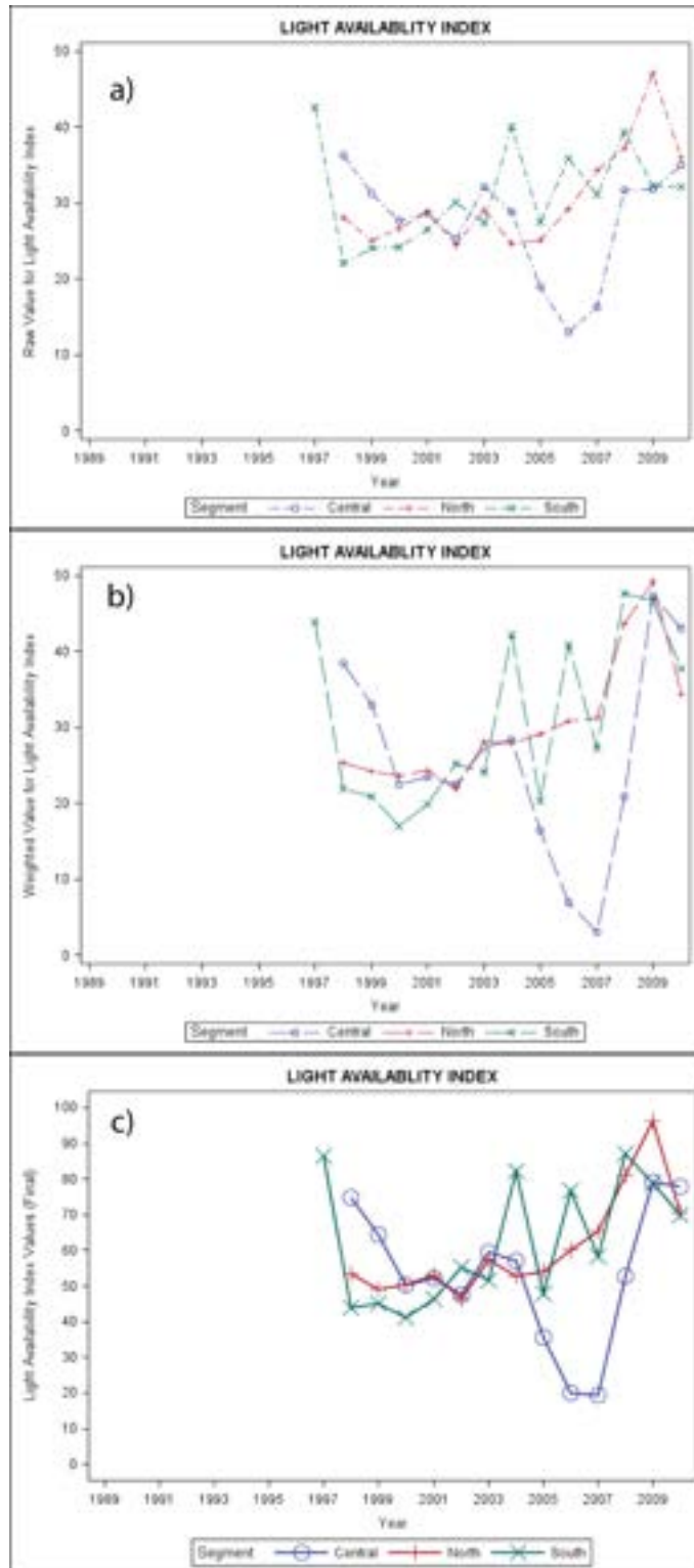
Figure 3 - 55 Light Availability Index scores: (a) Raw Scores, (b) Weighted Scores, (c) Final Scores.
