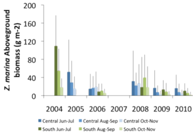
Figure 2 - 12 Mean aboveground eelgrass biomass values in the central and south segments of the BB-LEH Estuary during the spring-fall sampling periods from 2004 to 2010.
