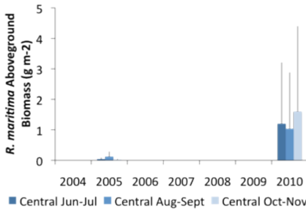
Figure 2 - 20 Mean aboveground widgeon grass biomass values in the central and south segments of the BB-LEH Estuary during the spring-fall sampling periods from 2004 to 2010.
