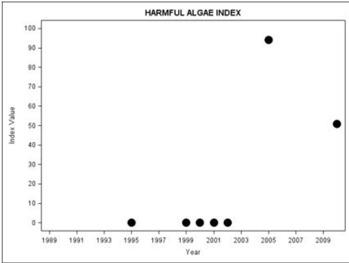
Figure 3 - 52 Harmful Algal Bloom Index.
