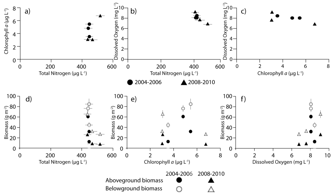
Figure 2 - 14 Variation of water quality and biological metrics for 2004-2006 (circles) and 2008-2010 (triangles). Eelgrass biomass is divided into aboveground (black) and belowground (white) components. Plots include chlorophyll a vs. total nitrogen (a), dissolved oxygen vs. total nitrogen (b), dissolved oxygen vs. chlorophyll a (c), eelgrass biomass vs. total nitrogen (d), eelgrass biomass vs. chlorophyll a (e), and eelgrass biomass vs. dissolved oxygen (f).
