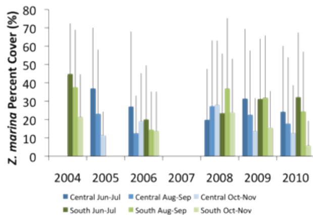
Figure 2 - 17 Mean eelgrass percent cover in the central and south segments of the BB-LEH during the spring-fall sampling periods from 2004 to 2010.
