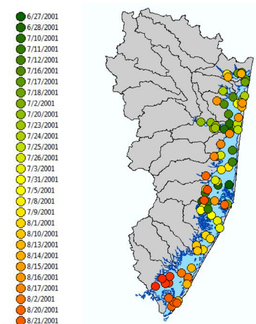
Figure 2 - 25 Benthic invertebrate sampling stations (2001) of the USEPA Regional Monitoring and Assessment Program for the BB-LEH Estuary.
