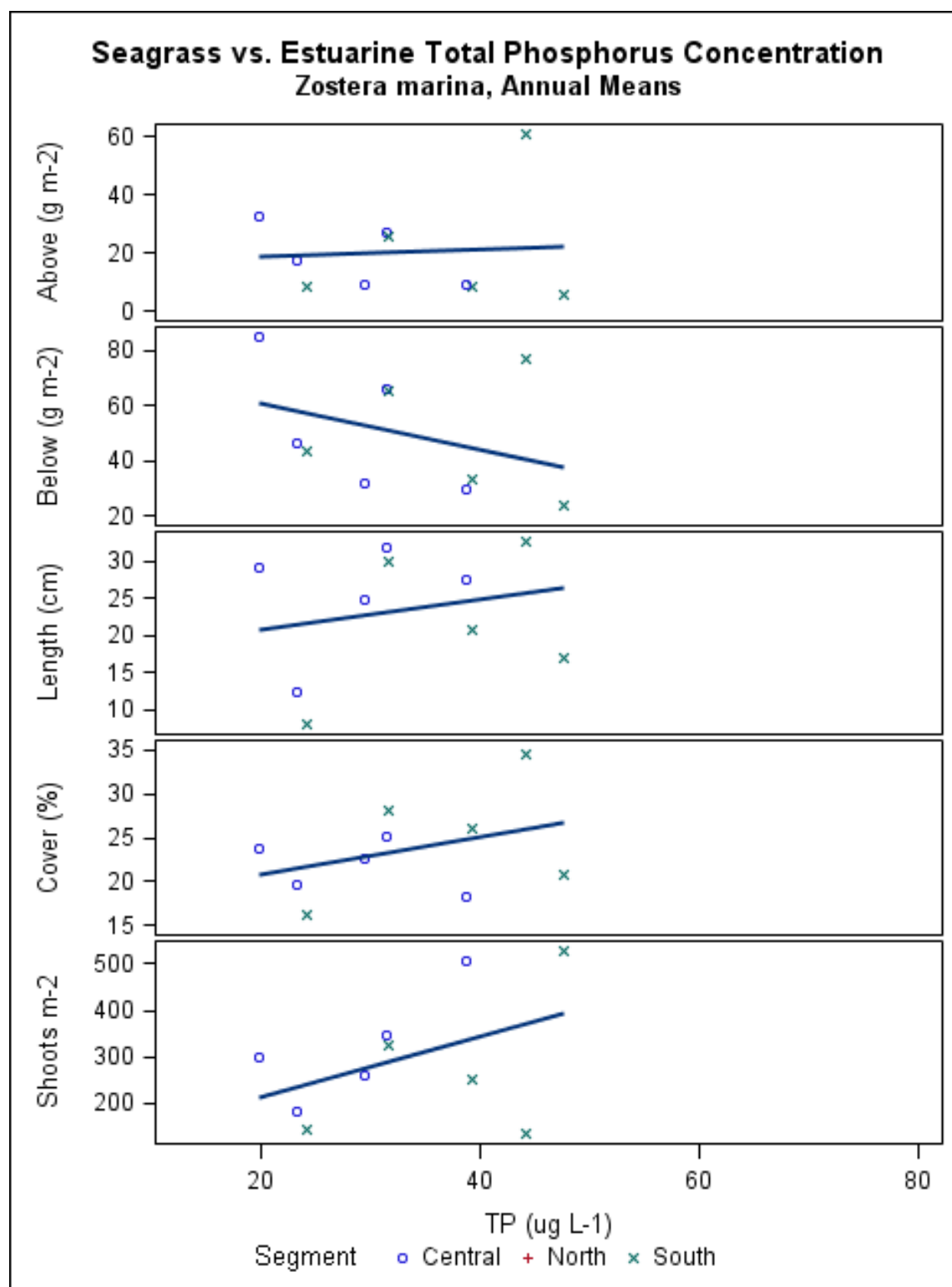
Figure 3 - 33 Seagrass indicators vs estuarine total phosphorus
