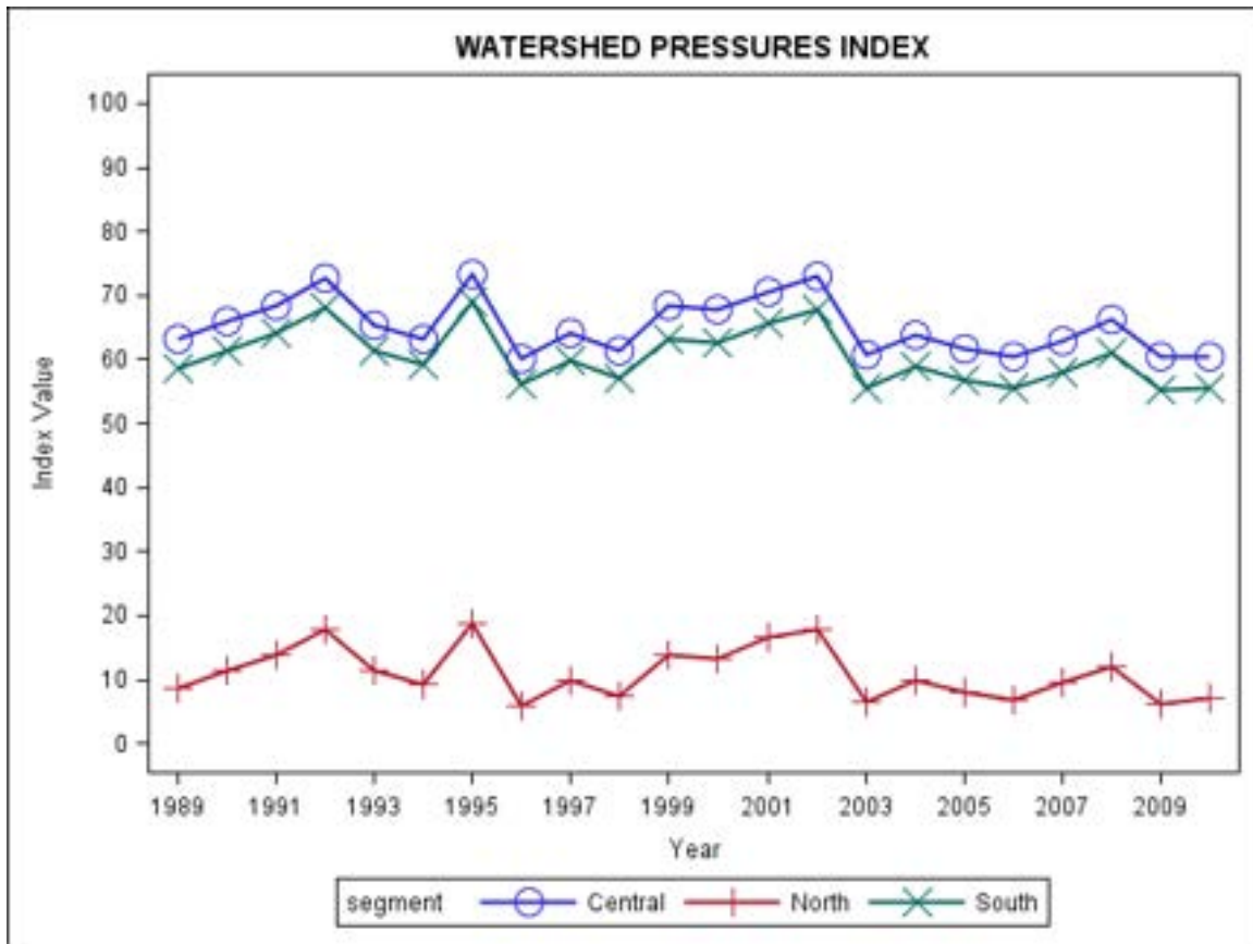
Figure 3 - 53 Watershed Pressure Index.
