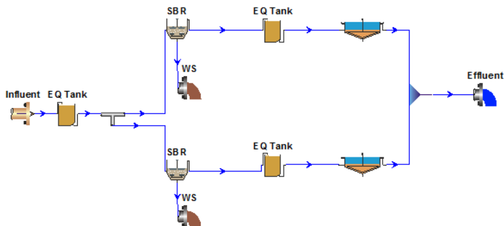
Figure B-3 Baseline Model, Belchertown, MA
