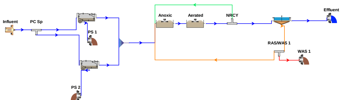
Figure GB-4 Conceptual Nitrogen Design Model, Great Barrington, MA
