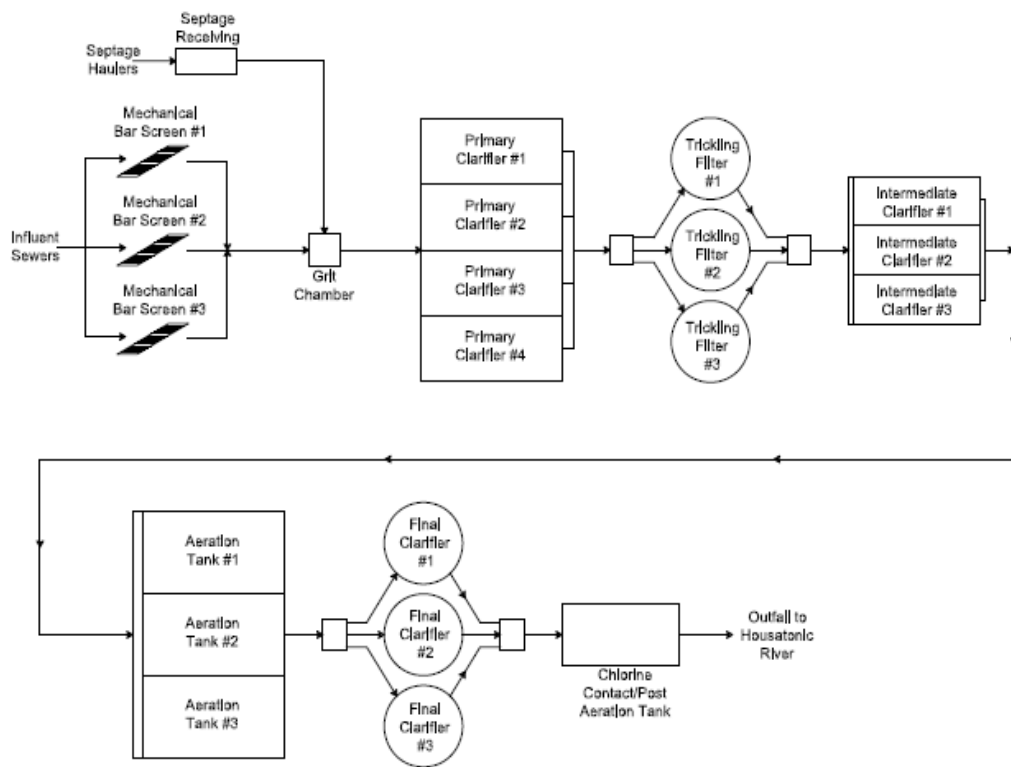
Figure PT-2 Pittsfield, MA, Process Flow Diagram
