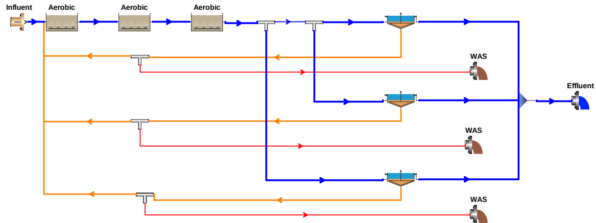
Figure W-3 Baseline Model, Webster, MA
