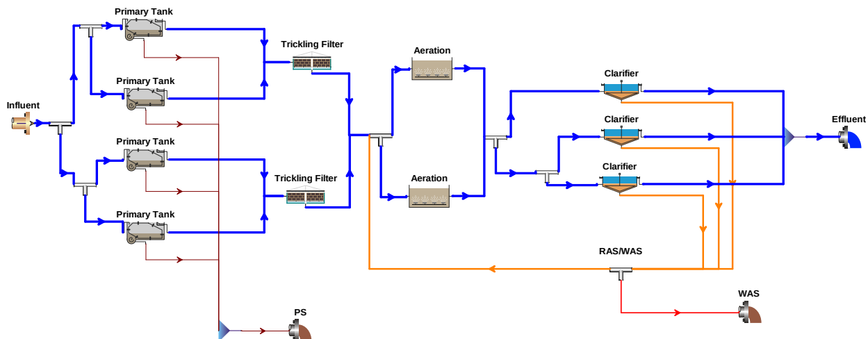
Figure PT-3 Baseline Model, Pittsfield, MA
