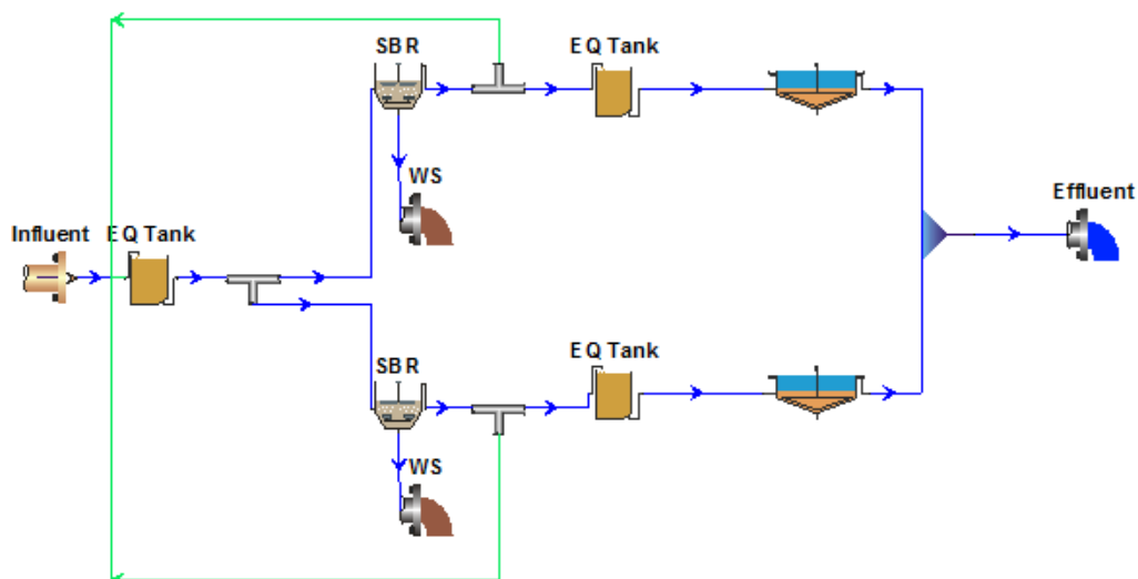
Figure B-4 Conceptual Nitrogen Design Model, Belchertown, MA
