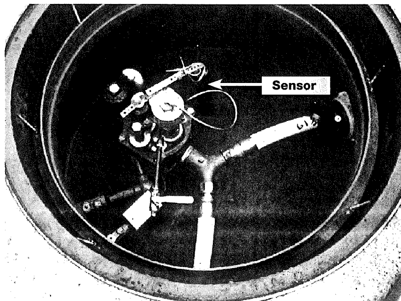
A properly installed float sensor.
