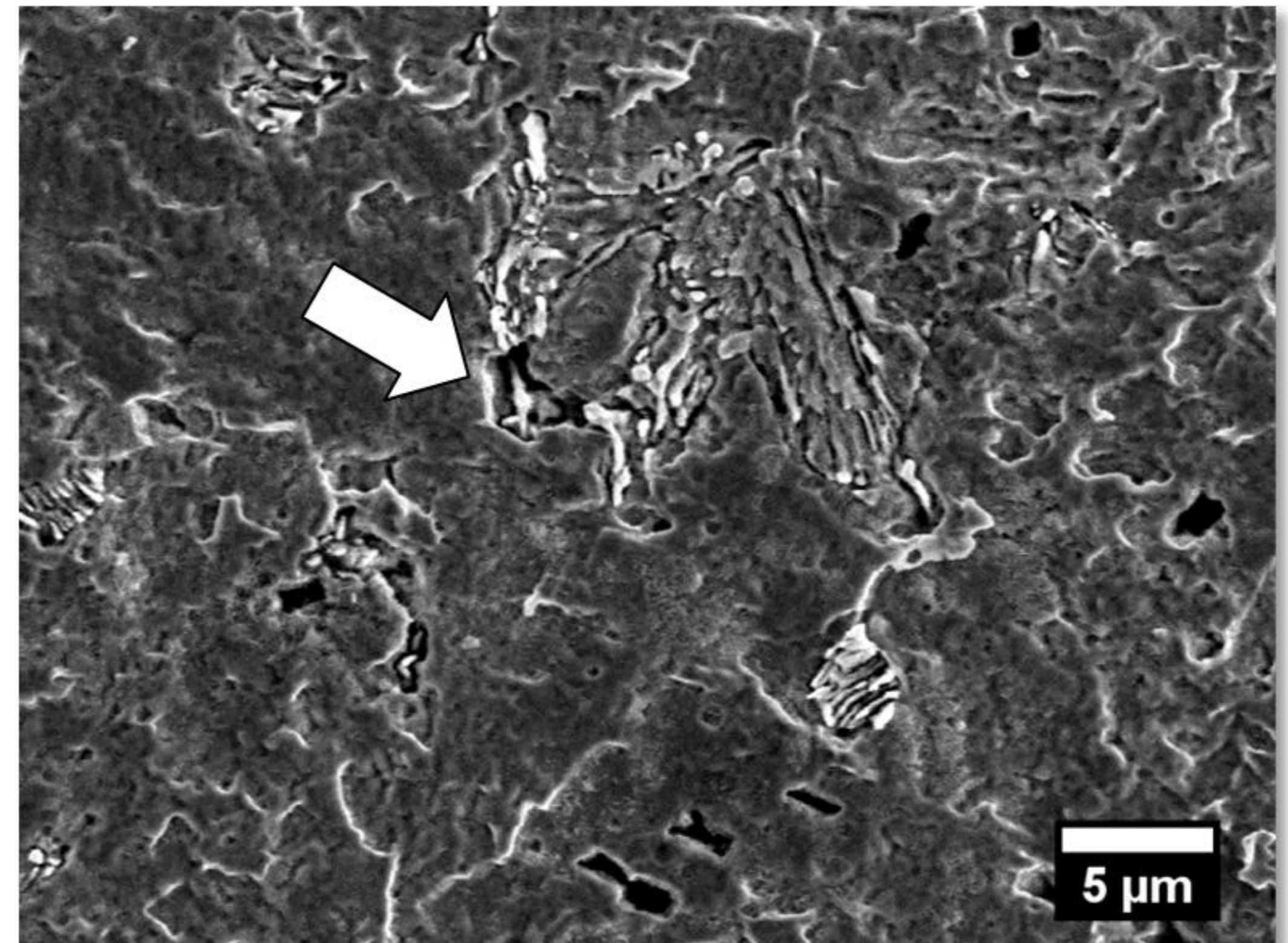
Pearlite Boundary Attack
