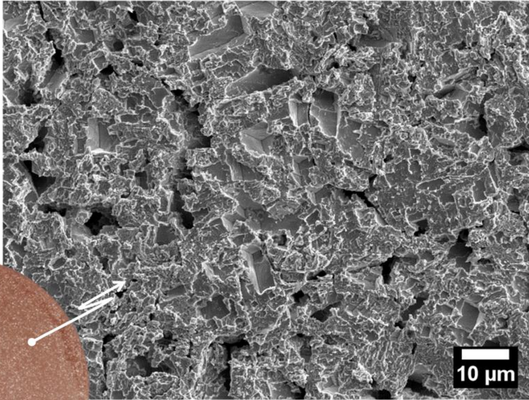
Intergranular Attack
