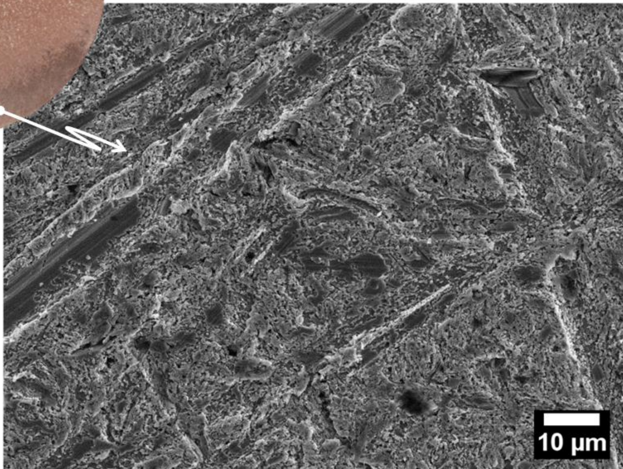
Fine Pitting In Scratches
