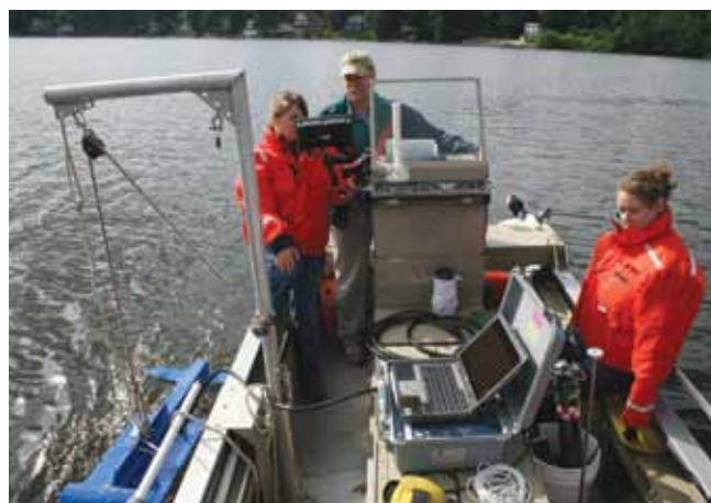
Preparing to deploy for a hydroacoustic survey.
